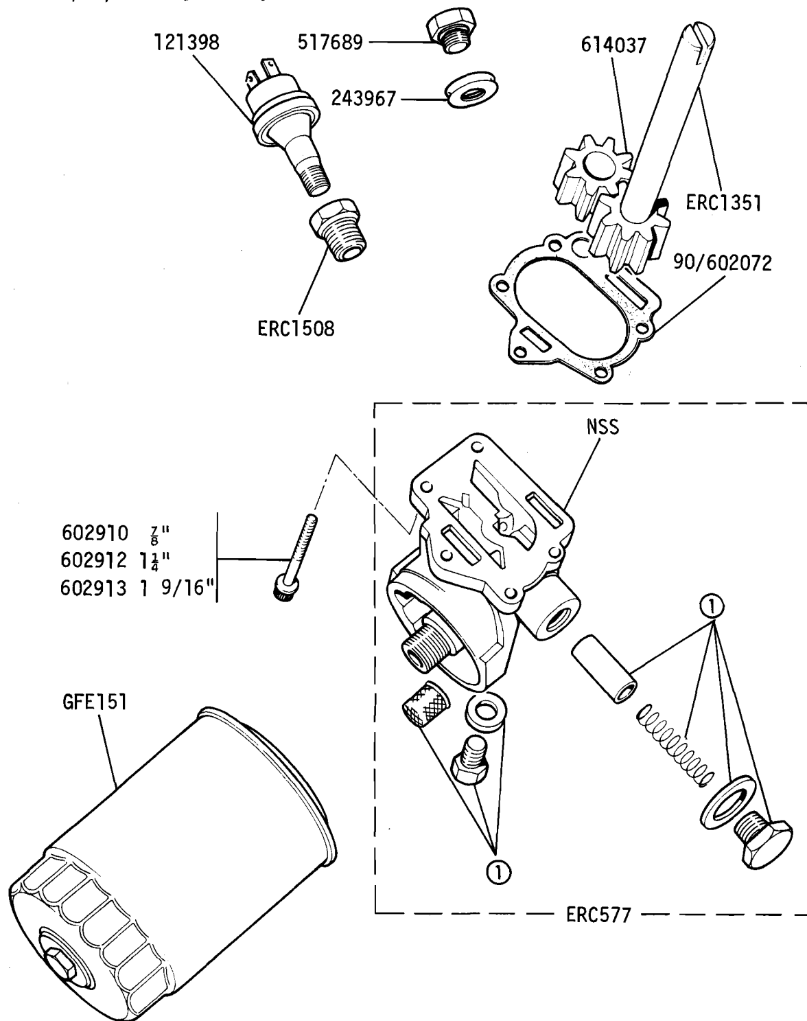
① RTC2044 Pressure relief kit
